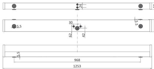
ELM66 1x36W
